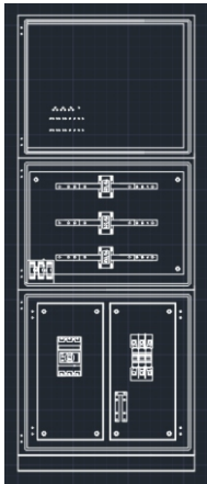
Part No – CTA - 630 Enclosure 800w x 2080h x 300d mm Suitable for single submain/ mains installations, ideal for supply upgrades.
