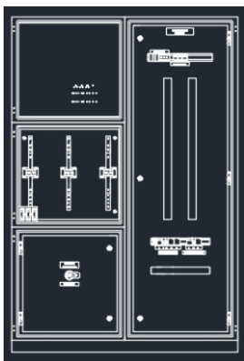
Part No CT-630 Enclosure 1400w x 2080h x 400d mm Suitable for all types of CT metering, large distribution section suitable for MCB MCCB Chassis
